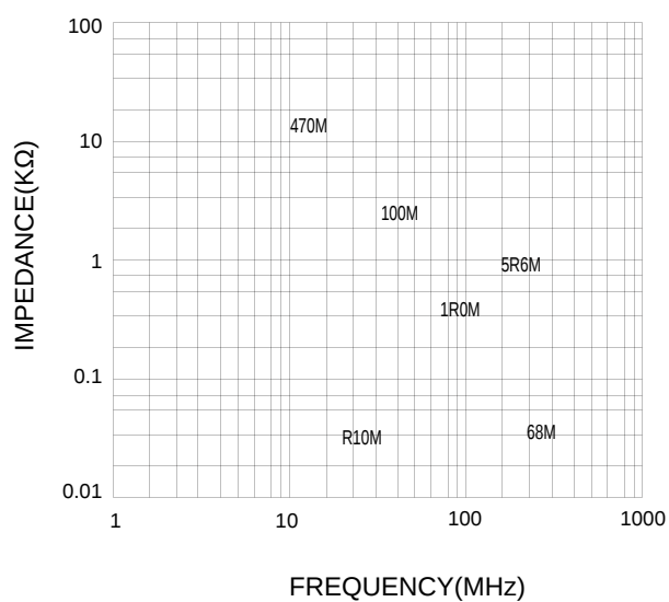
Impedance VS. Frequency Characteristics:1010
